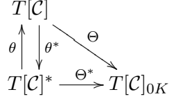
Figure 5: Relationships between T[\mathcal{C}] , T[\mathcal{C}]^* and T[\mathcal{C}]_{0K} .
