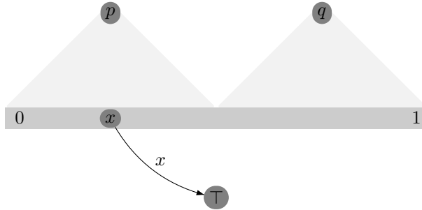
Figure 1: The two states p and q do not simulate each other, but they satisfy the same formulas of \text{PML}_{\forall} .
