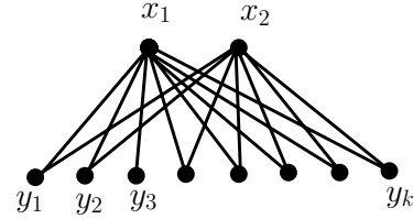
Figure 6: In this example, we have a complete bipartite graph B = (X, Y, E) where X = \{x_1, x_2\} and Y = \{y_1, \dots, y_k\} . We set the connectivity requirements between y_i and y_j to be 1 for all i, j , between x_1 and x_2 to be \frac{k}{2} , and 0 otherwise. The fractional solution where all edges have fractional value \frac{1}{2} is the optimal solution, in which the degree of x_1 and x_2 is equal to \frac{k}{2} = \Delta_f^* . On the other hand, it can be seen that in any integer solution, the degree of x_1 and x_2 must be at least \frac{3}{4}k = \frac{3}{2}\Delta_f^* . This example also shows that the integrality gap is at least (2, B_v + \frac{r_{max}}{2}) .
