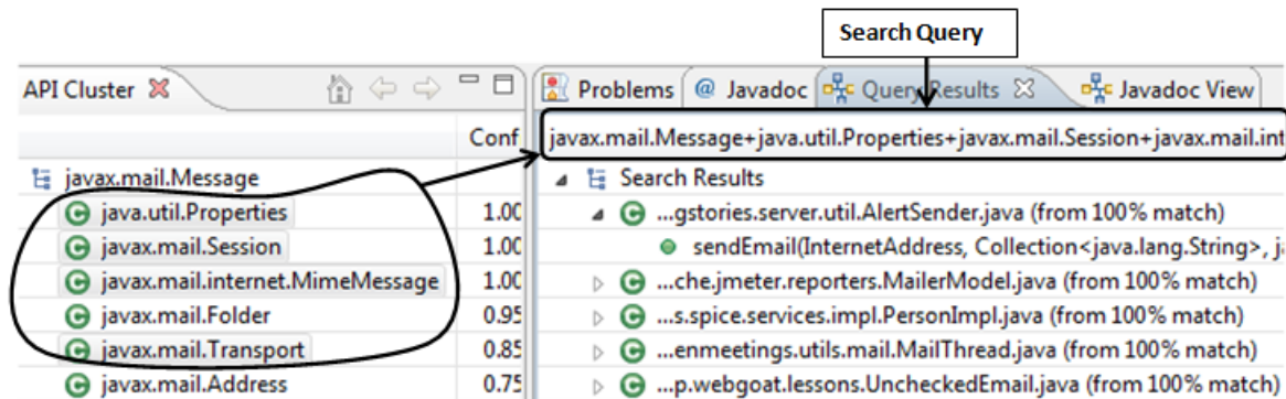
Figure 1–6: Formulating a search query from the recommendations of Introspector.
