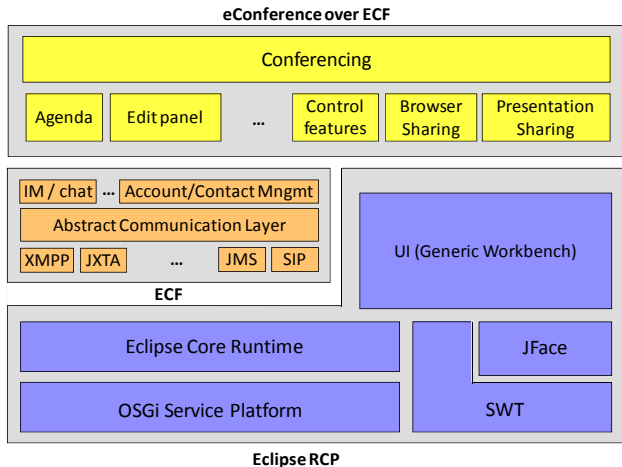
Figure 2. The 4th generation of eConference is a rich client application composed by ad hoc and ECF-native plugins
