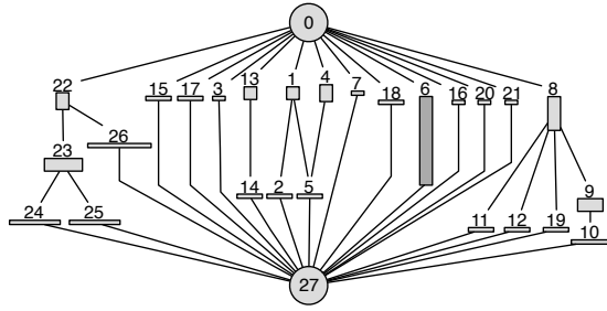
Figure 3. Hierarchy of blocks from an Eclipse transaction. Labels identify blocks but otherwise are arbitrary. Block 6 is an aspect candidate of size 14 \times 1 , cross-cutting 14 locations.
