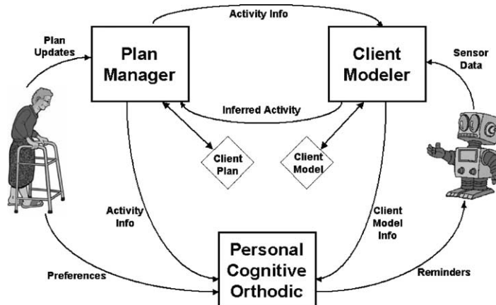
Fig. 2. Autominder architecture.
