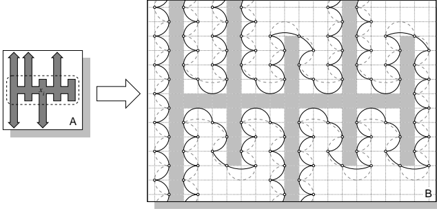
Figure 3: The point set P_x representing the vertex x and all adjacent edges in the P3SAT graph. The grey strips extending out of the frame in (B) represent edges going from x to clause vertices. A_x and A'_x are shown in (B) outlining the shape of the gadget.
