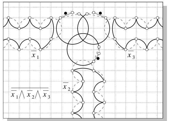
Figure 6: clause x_1 \vee x_2 \vee x_3 \equiv \overline{x_1} \wedge \overline{x_2} \wedge \overline{x_3}
