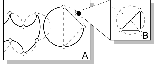
Figure 5: (A) clause gadget component and (B) blocking gadget
