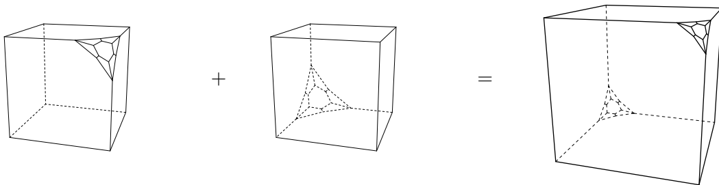
Figure 1: A construction of “easy” Minkowski addition problems
