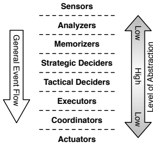
Figure 1: The Layered AI Model Architecture
