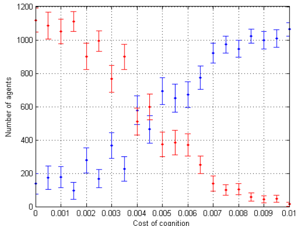
Figure 2: Number of ethnocentric and humanitarian agents vs. cost of cognition. The points represent the mean number of agents over the last 500 cycles of the simulations: red is ethnocentric agents, blue is humanitarian. The error bars represent standard error from averaging over 30 different worlds.
