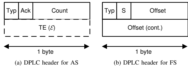
Fig. 5: DPLC data packet headers for AS and FS.
