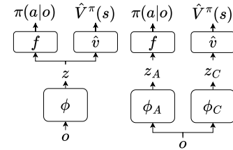
Figure 1: Models with shared (left) and decoupled representations (right).
