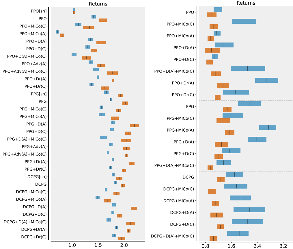
Figure 13: Returns in Procgen (left) and Brax (right).
