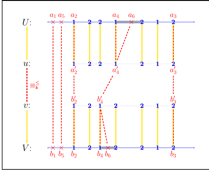
Fig. 1. Visualization of the Duplicator's strategy in the proof of Theorem 4.1 with u = 1221212 and v = 1212212 . U and V are padded versions of u and v ; (multiple) occurrences of the letter e are visualized by a solid line between the letters 1 and 2.
